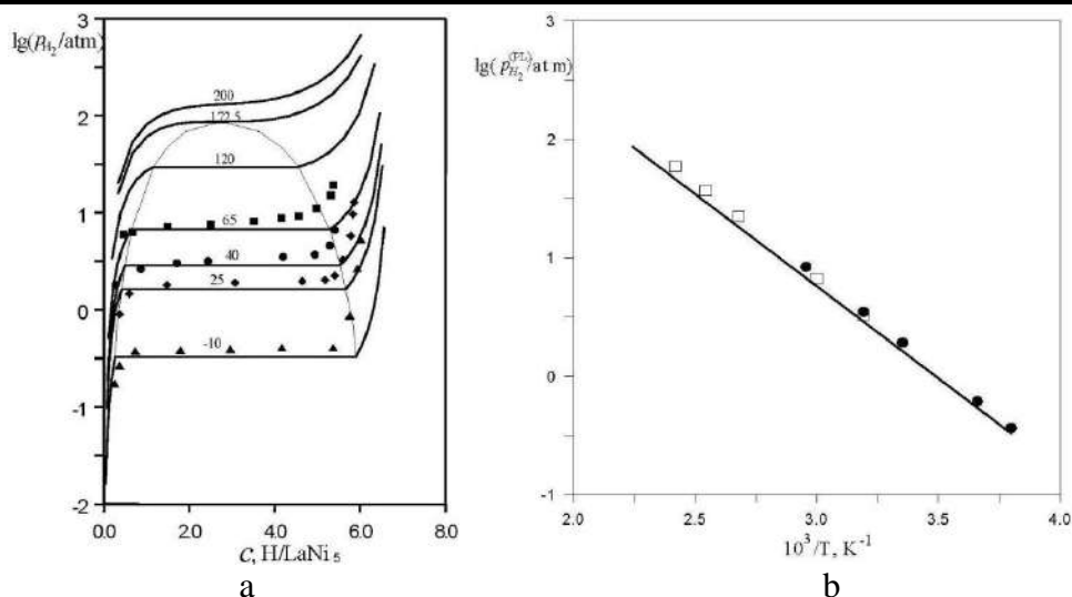
Fig. 1. Hydrogen solubility isotherms p_{H_2} (C) in the LaNi_5 compound at T < T_c and T \geq T_c (a) (temperatures at calculated isotherms are indicated in °C, the dotted curve is the calculated boundaries of one- and two-phase regions in the plane ( \log p_{H_2} - C ), symbols – experimental data on desorption); Logarithm of the decomposition pressure of the \beta -phase of LaNi_5 hydrides as a function of inverse temperature (b) (calculation according at \Delta H_{\beta \rightarrow \alpha} = 29,8 \text{ kJ/mol H}_2 , \Delta S_{\beta \rightarrow \alpha} = 104 \text{ J/(K}\cdot\text{mol H}_2 Symbols – experimental data on desorption in the LaNi_5 - H_2 system).
